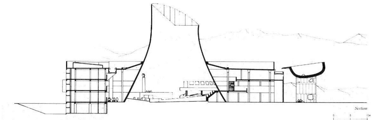
Le Corbusier, Palace of Assembly, Chandigarh. Completed in 1963. Transversal Section
